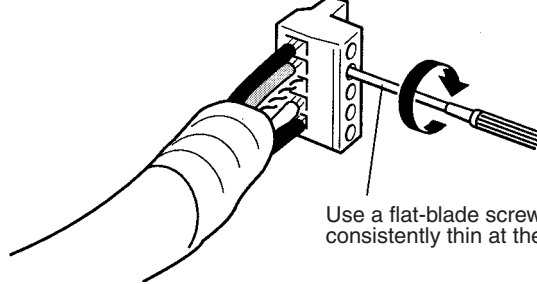
Connector without Set Screws
