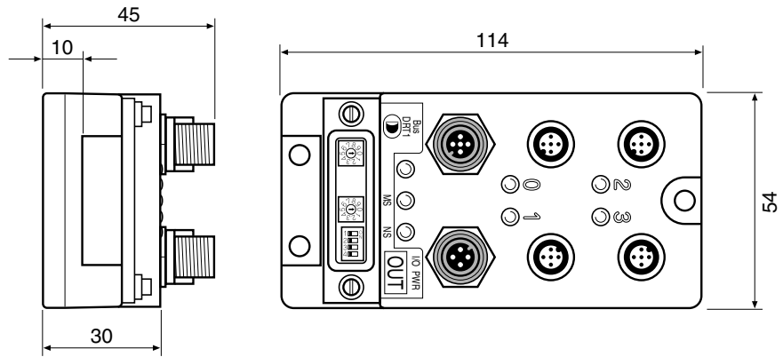
Mounting holes
