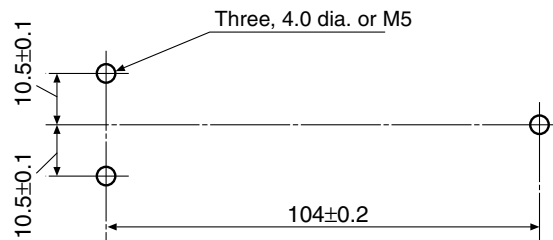
Mounting holes
