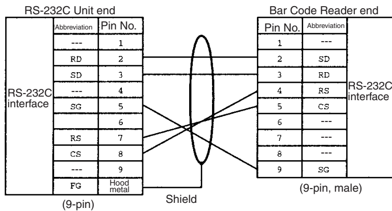
Connecting an OMRON V500-R32□ Bar Code Reader
