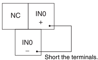
DRT2-TS04T Thermocouple input
