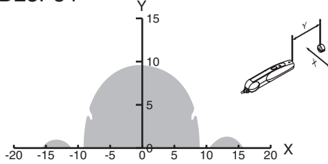
V600-D23P61
